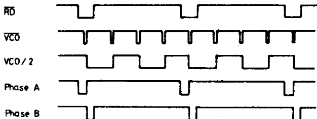
Diagramm 4 VCO = 1 MHz, RD = 250 kHz = Dateninformation "0"
