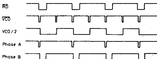
Diagramm 3 VCO = 760 kHz, RD = 380 kHz
