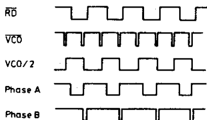
Diagramm 2 VCO = 1,44 MHz, RD = 720 kHz
